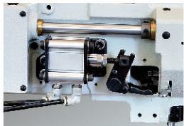
PF: 汽動抬壓腳 PF: Pneumatic foot lifter
